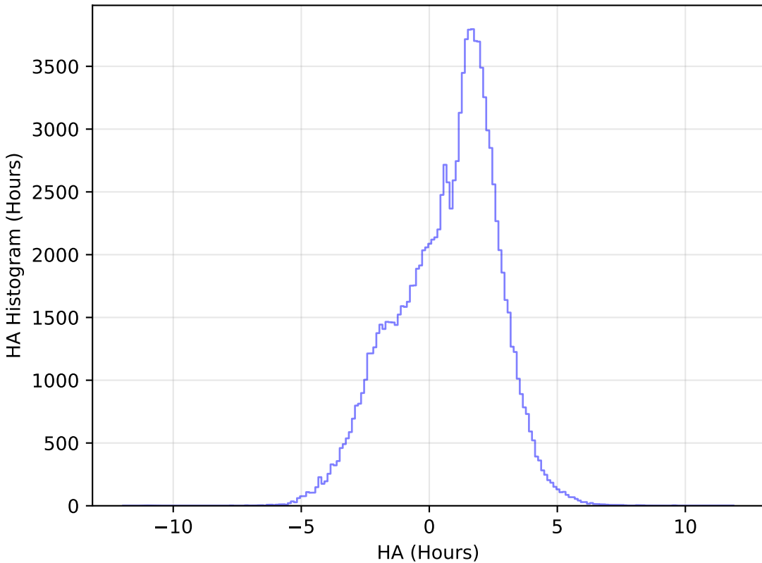
too_ignore_10_1v3.4_10yrs WFD u band: HA Histogram
