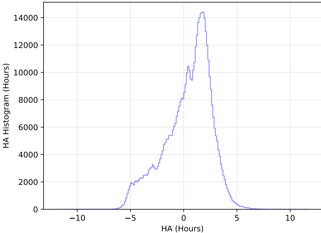
too_ignore_10_1v3.4_10yrs WFD r band: HA Histogram
