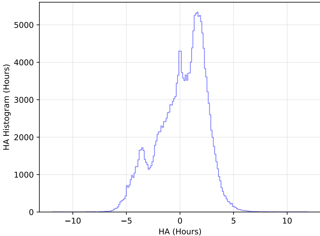
too_ignore_10_1v3.4_10yrs WFD g band: HA Histogram
