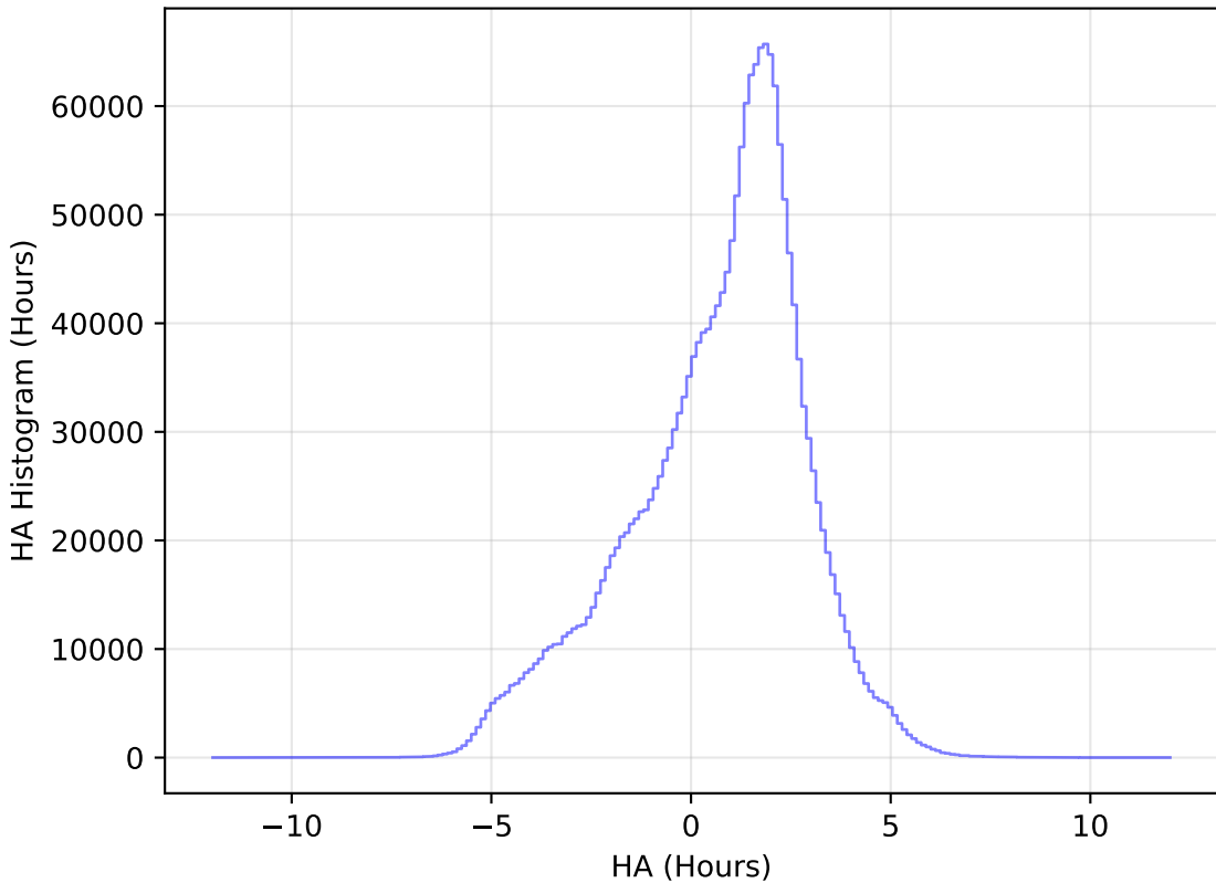
too_ignore_10_1v3.4_10yrs WFD all bands: HA Histogram
