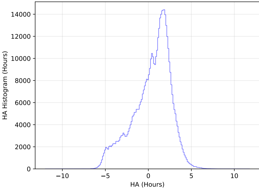
too_ignore_10_1v3.4_10yrs All sky r band: HA Histogram
