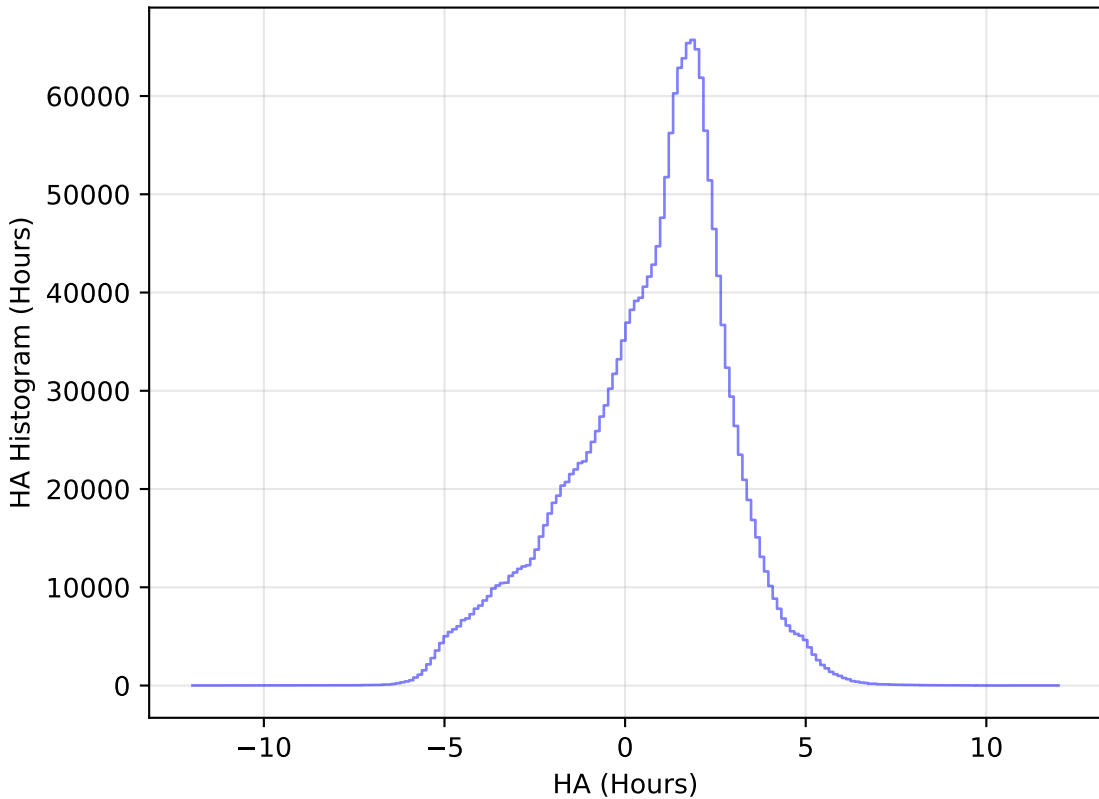
too_ignore_10_1v3.4_10yrs All sky all bands: HA Histogram
