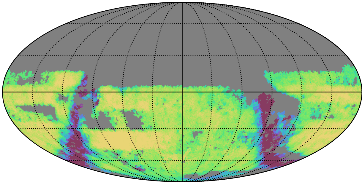
too_ignore_10_1v3.4_10yrs Yr 3-4 u band: Exgal_CoaddM5
