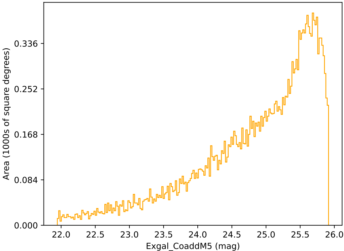
too_ignore_10_1v3.4_10yrs Yr 3-4 r band: Exgal_CoaddM5
