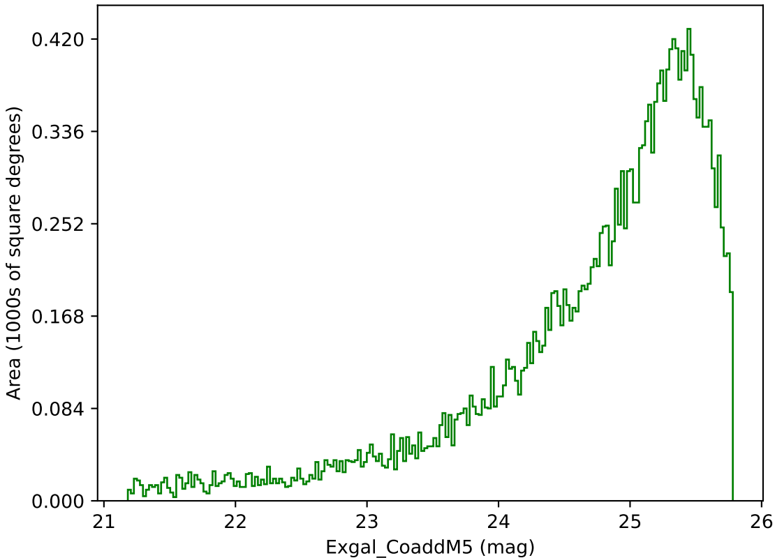
too_ignore_10_1v3.4_10yrs Yr 3-4 g band: Exgal_CoaddM5
