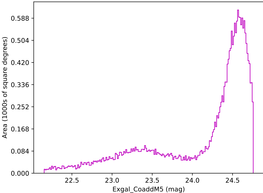
too_ignore_10_1v3.4_10yrs Yr 1 z band: Exgal_CoaddM5
