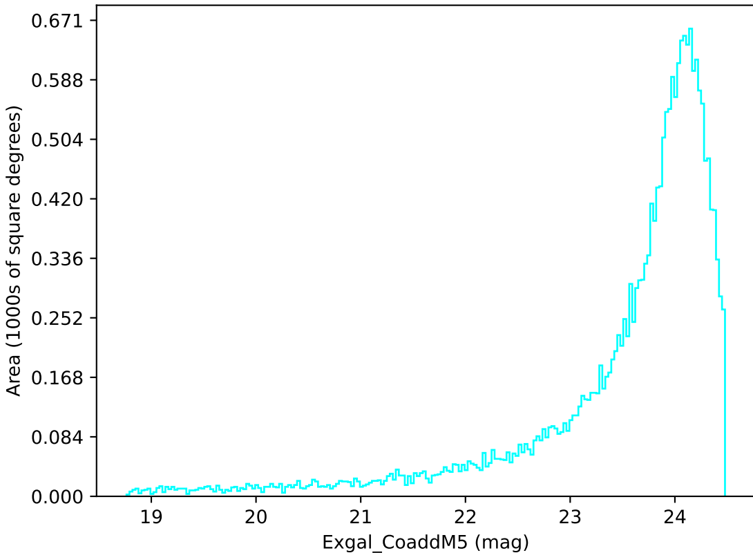
too_ignore_10_1v3.4_10yrs Yr 1 u band: Exgal_CoaddM5
