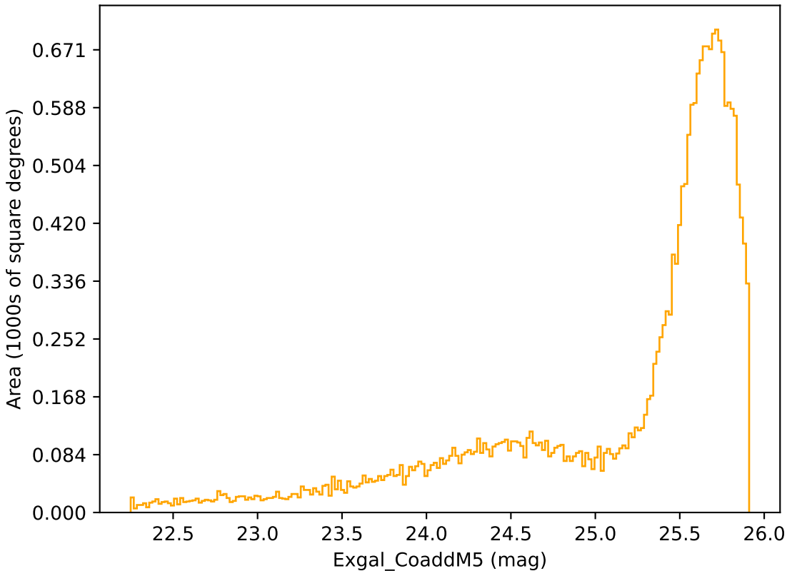
too_ignore_10_1v3.4_10yrs Yr 1 r band: Exgal_CoaddM5
