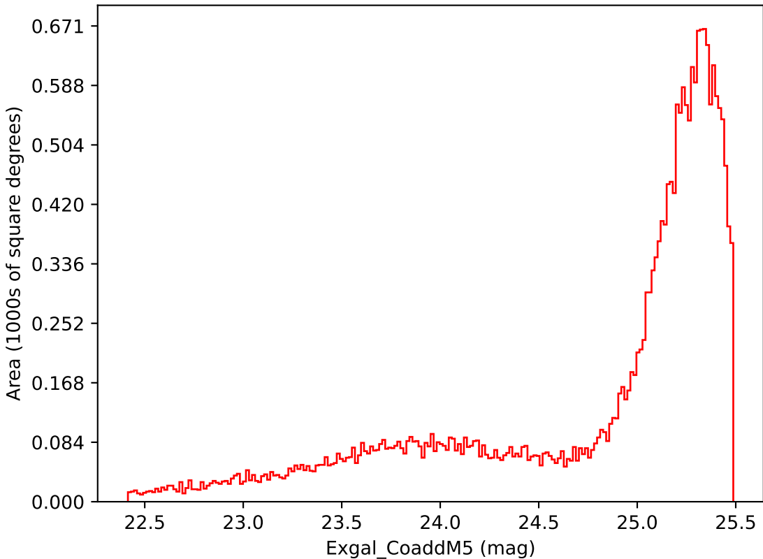
too_ignore_10_1v3.4_10yrs Yr 1 i band: Exgal_CoaddM5
