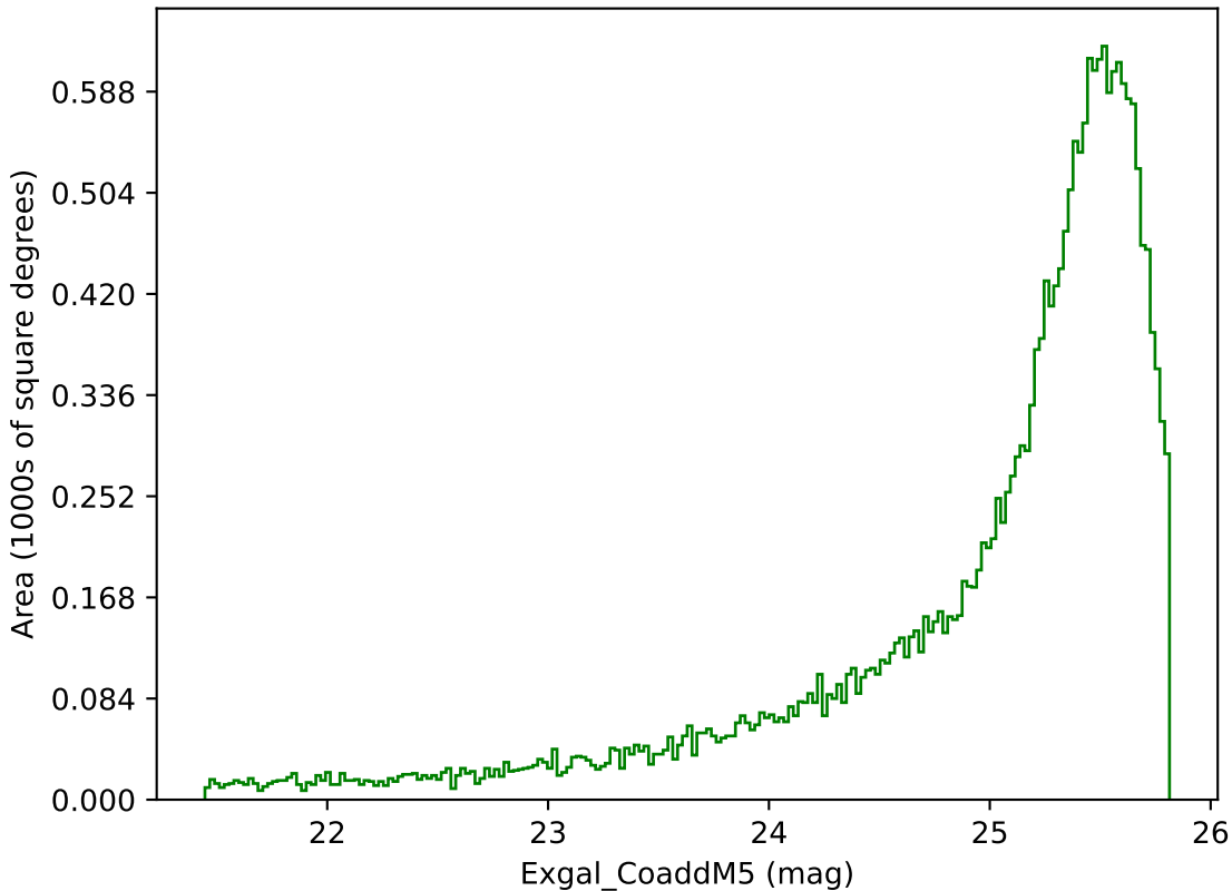
too_ignore_10_1v3.4_10yrs Yr 1 g band: Exgal_CoaddM5
