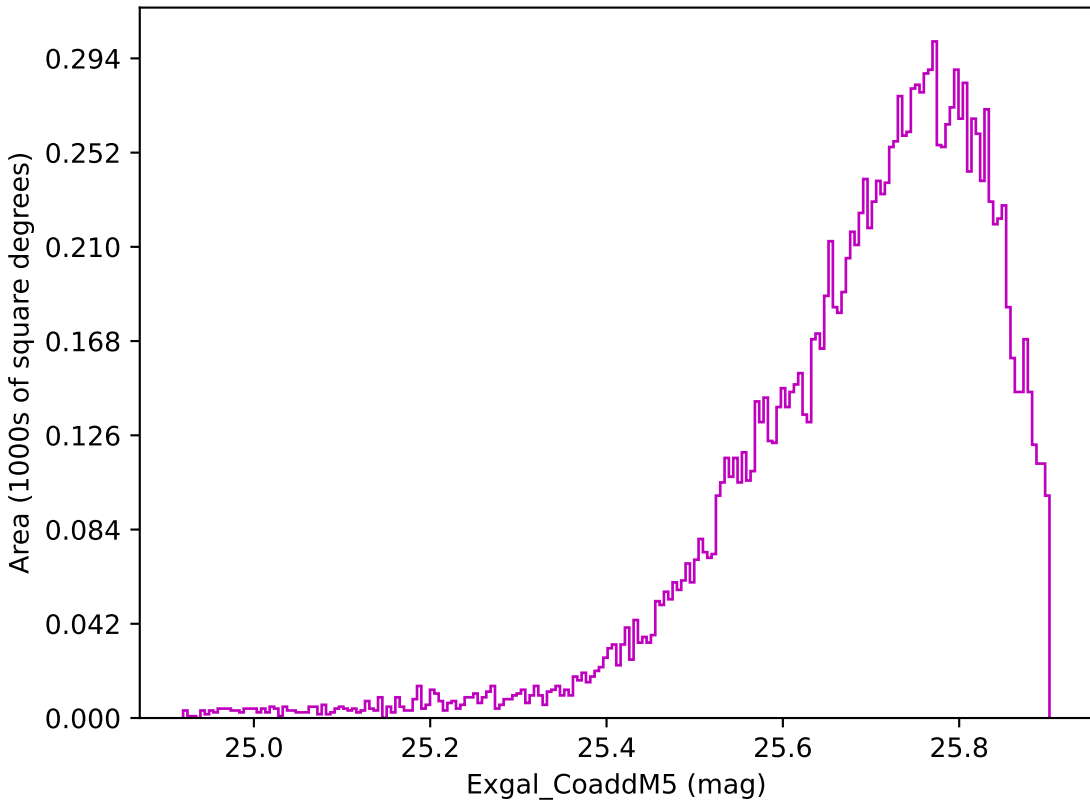
too_ignore_10_1v3.4_10yrs WFD z band: Exgal_CoaddM5
