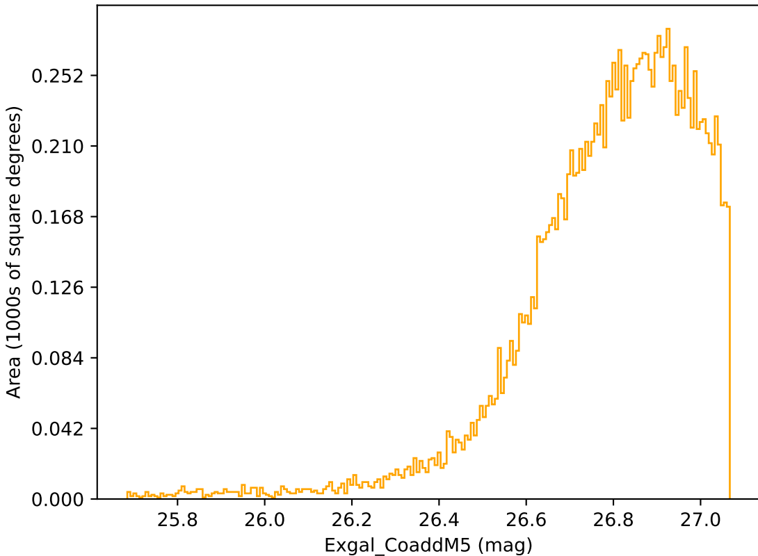
too_ignore_10_1v3.4_10yrs WFD r band: Exgal_CoaddM5
