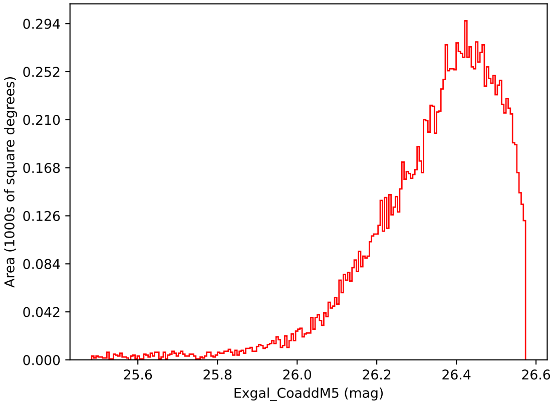
too_ignore_10_1v3.4_10yrs WFD i band: Exgal_CoaddM5
