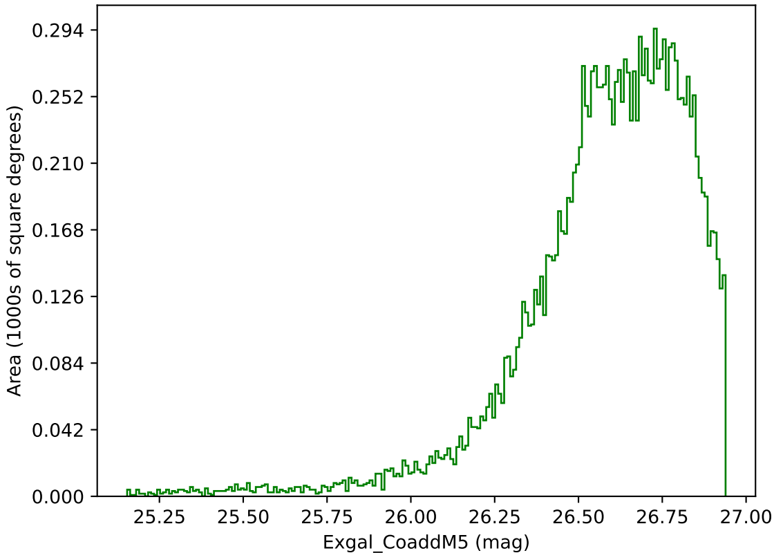
too_ignore_10_1v3.4_10yrs WFD g band: Exgal_CoaddM5
