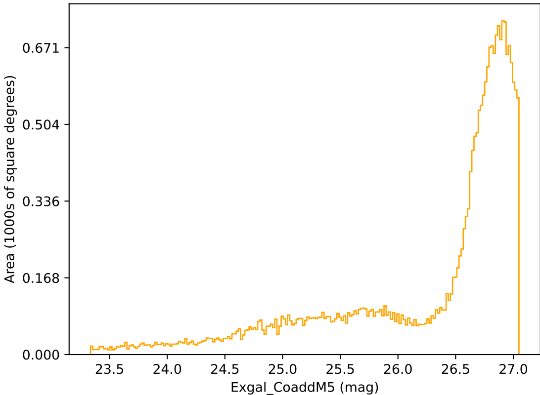
too_ignore_10_1v3.4_10yrs All sky r band: Exgal_CoaddM5
