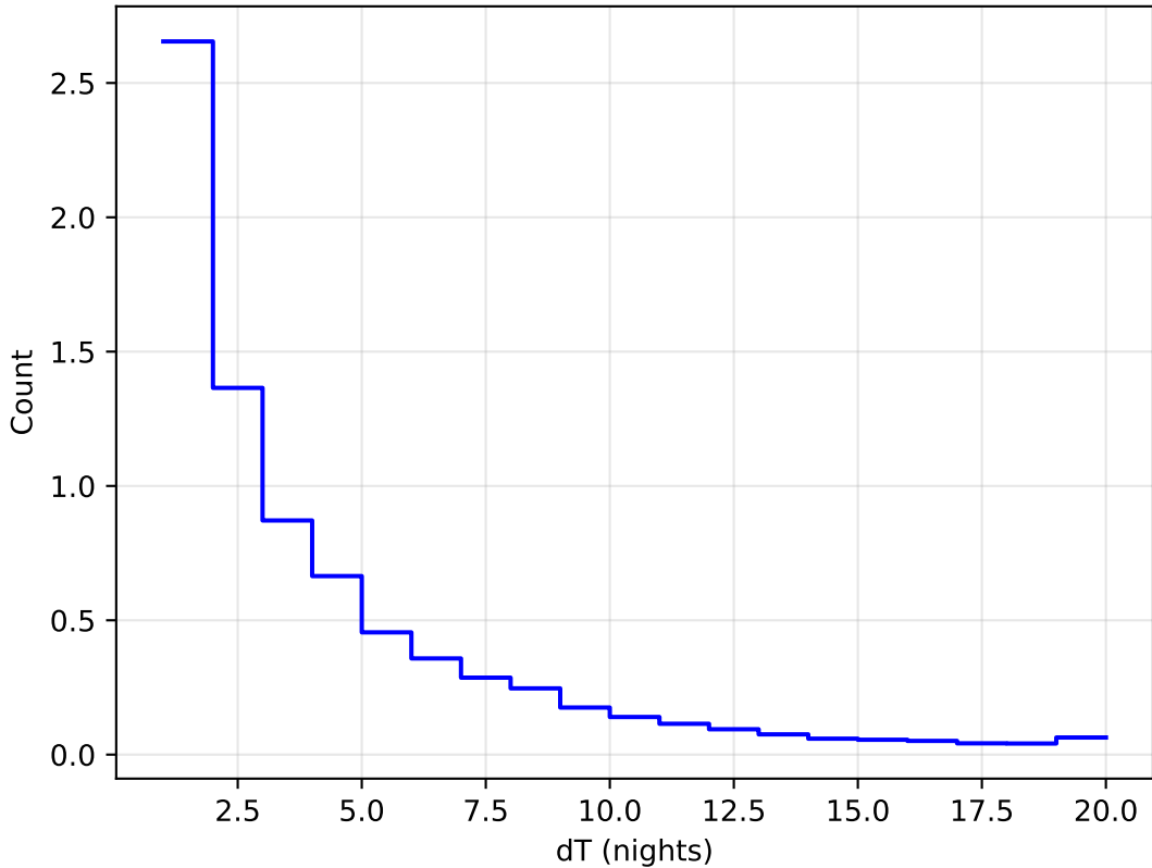
too_ignore_10_1v3.4_10yrs WFD all bands: DeltaNight Histogram 1e6
