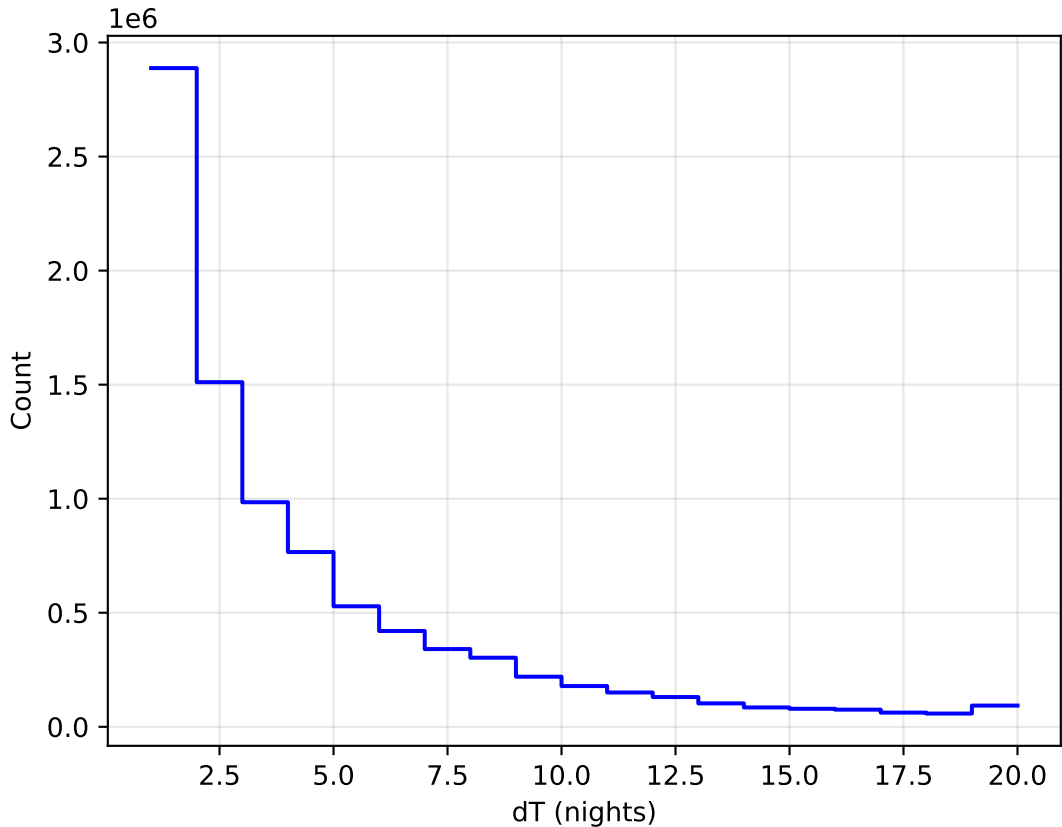
too_ignore_10_1v3.4_10yrs All sky all bands: DeltaNight Histogram
