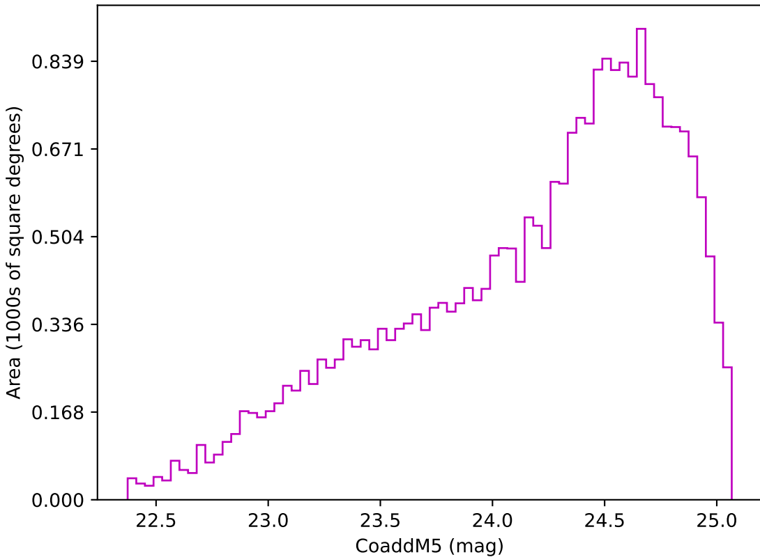
too_ignore_10_1v3.4_10yrs Yr 3-4 z band: CoaddM5
