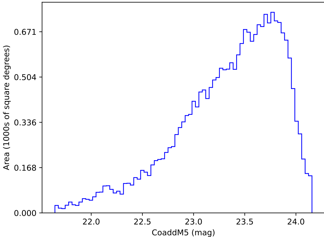
too_ignore_10_1v3.4_10yrs Yr 3-4 y band: CoaddM5
