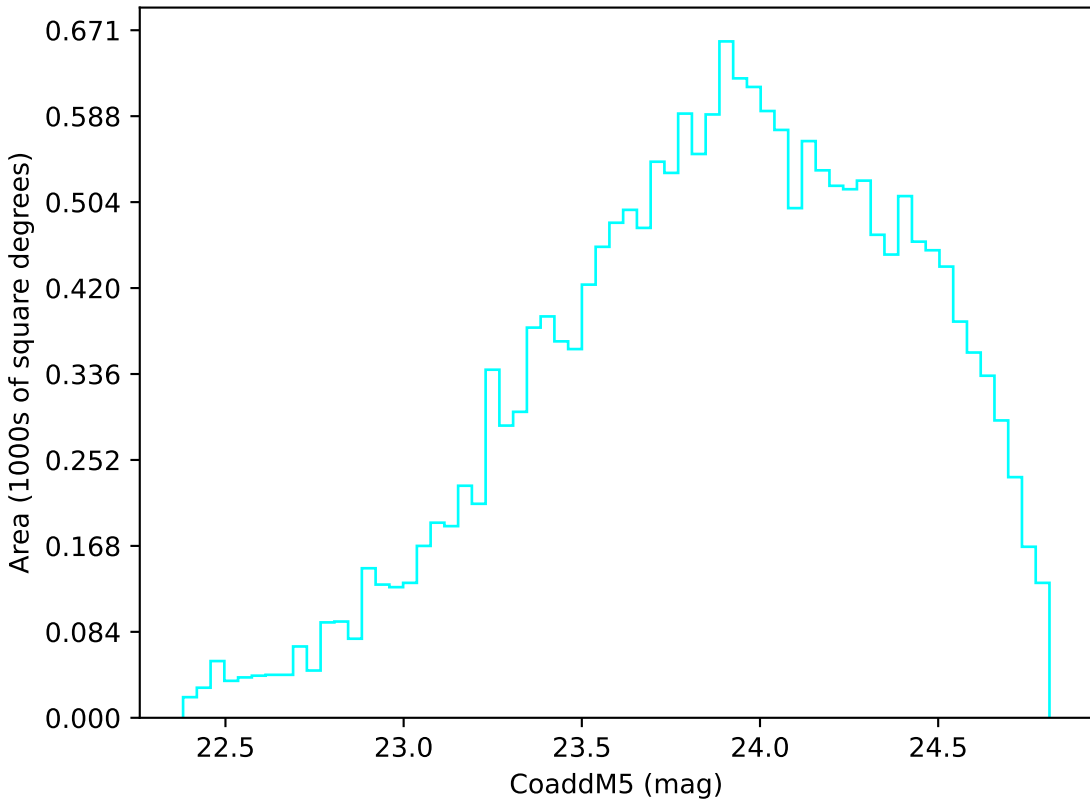
too_ignore_10_1v3.4_10yrs Yr 3-4 u band: CoaddM5
