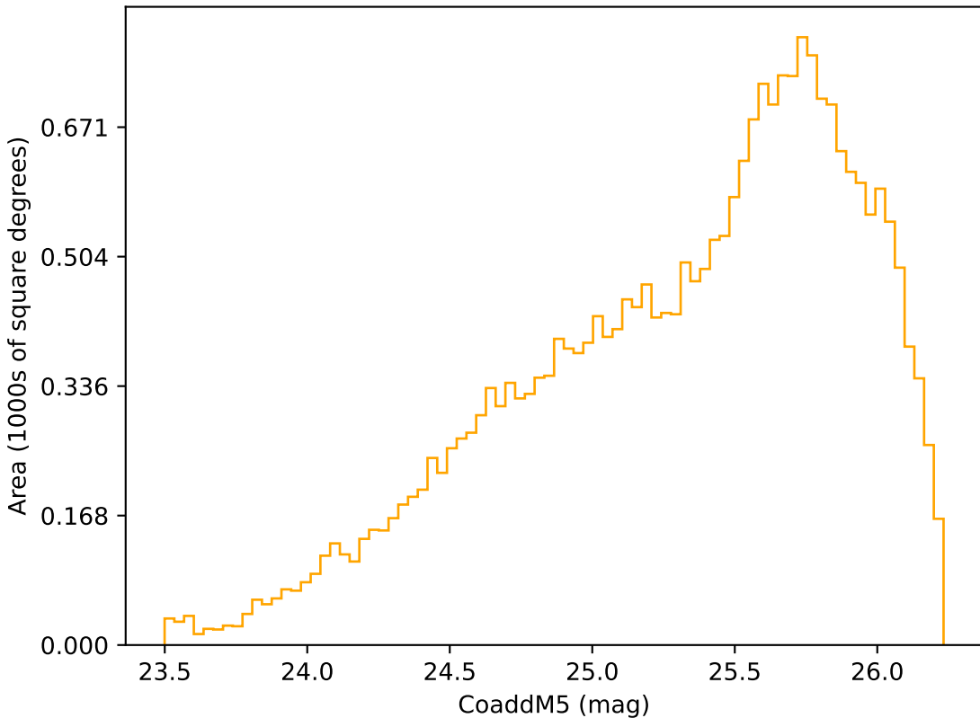
too_ignore_10_1v3.4_10yrs Yr 3-4 r band: CoaddM5
