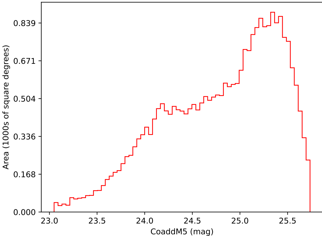
too_ignore_10_1v3.4_10yrs Yr 3-4 i band: CoaddM5
