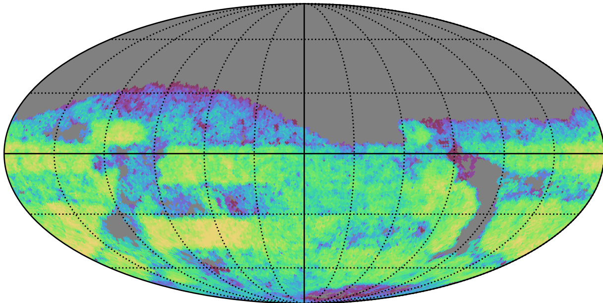
too_ignore_10_1v3.4_10yrs Yr 3-4 g band: CoaddM5
