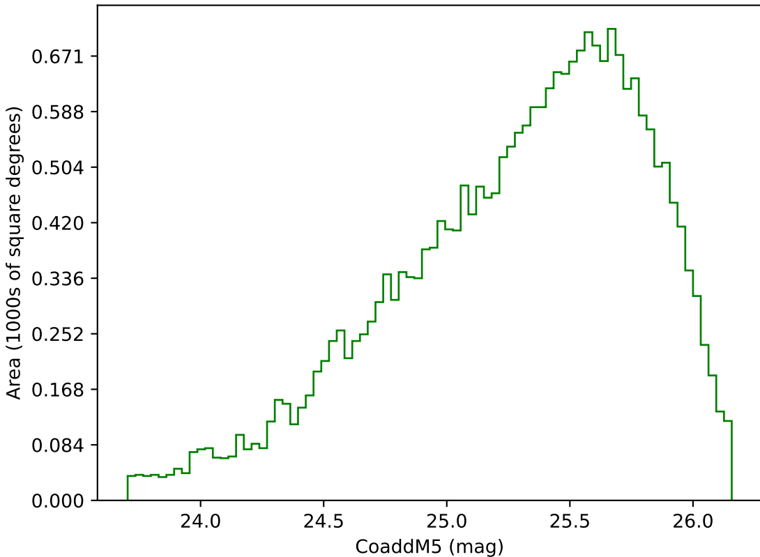
too_ignore_10_1v3.4_10yrs Yr 3-4 g band: CoaddM5
