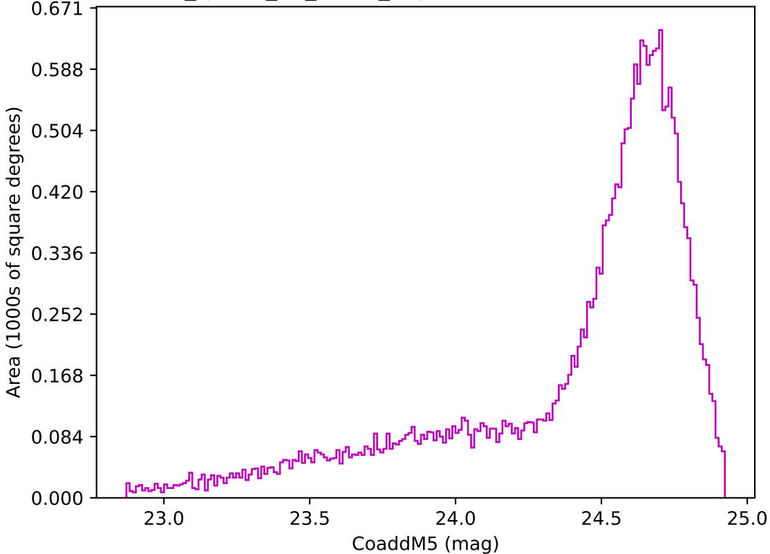
too_ignore_10_1v3.4_10yrs Yr 1 z band: CoaddM5
