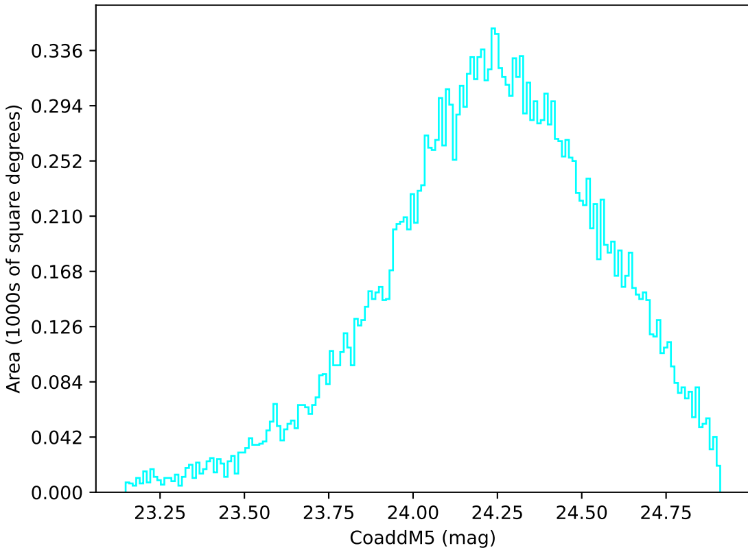
too_ignore_10_1v3.4_10yrs Yr 1 u band: CoaddM5
