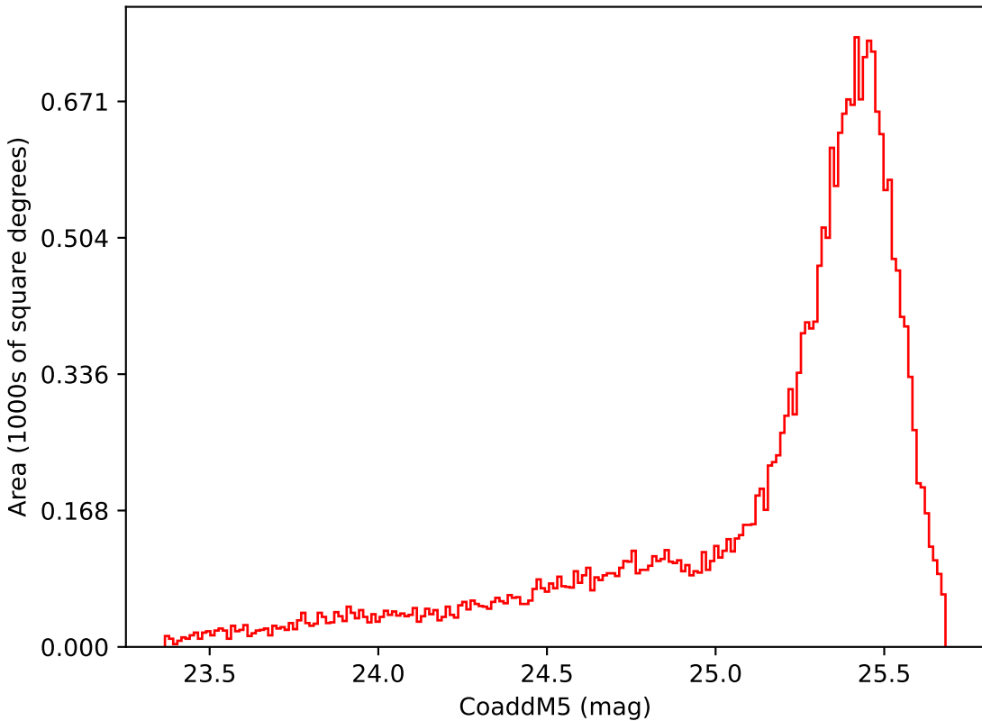
too_ignore_10_1v3.4_10yrs Yr 1 i band: CoaddM5
