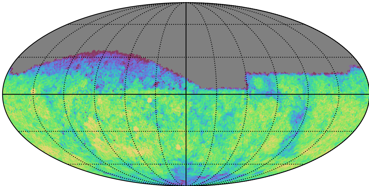
too_ignore_10_1v3.4_10yrs Yr 1 g band: CoaddM5
