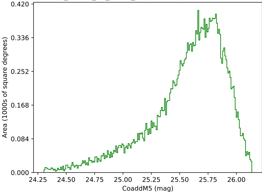
too_ignore_10_1v3.4_10yrs Yr 1 g band: CoaddM5
