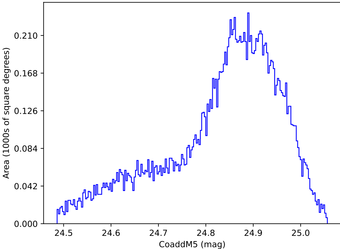
too_ignore_10_1v3.4_10yrs WFD y band: CoaddM5
