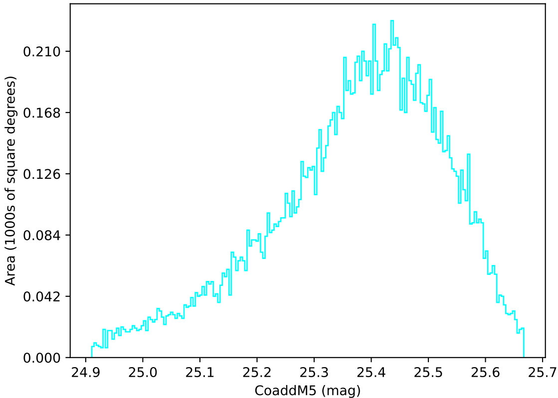
too_ignore_10_1v3.4_10yrs WFD u band: CoaddM5
