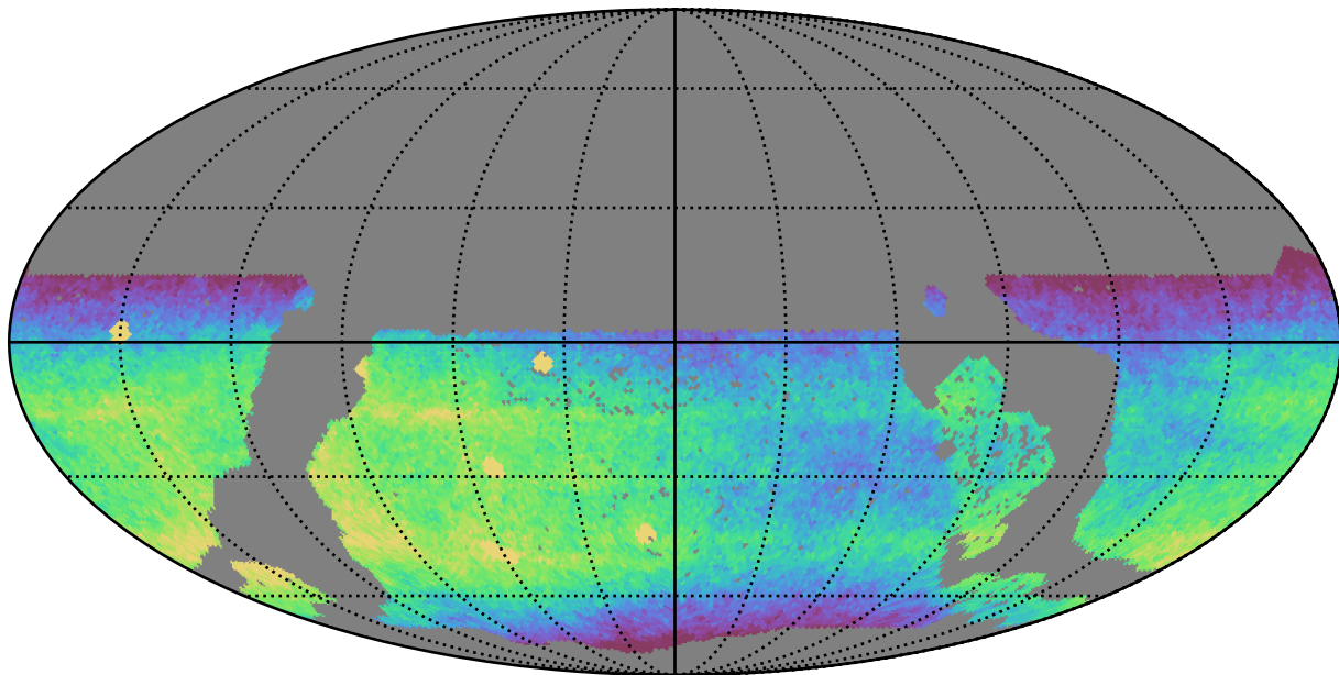
too_ignore_10_1v3.4_10yrs WFD r band: CoaddM5
