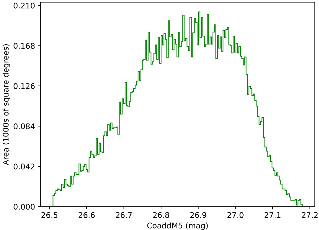
too_ignore_10_1v3.4_10yrs WFD g band: CoaddM5
