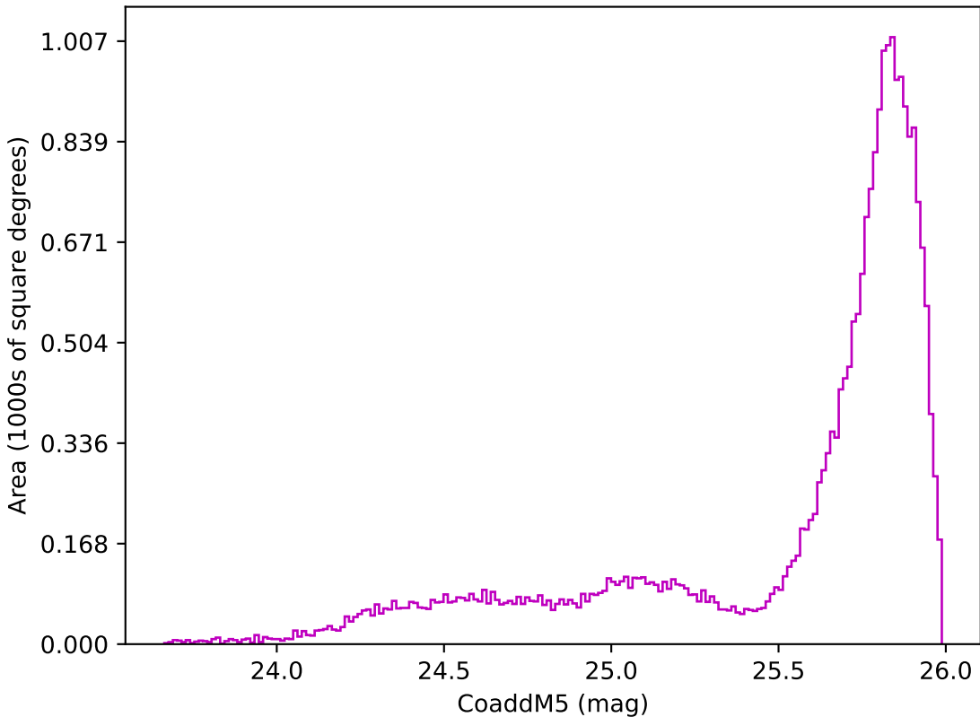
too_ignore_10_1v3.4_10yrs All sky z band: CoaddM5
