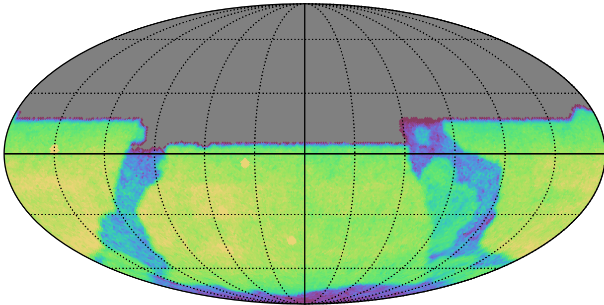
too_ignore_10_1v3.4_10yrs All sky u band: CoaddM5
