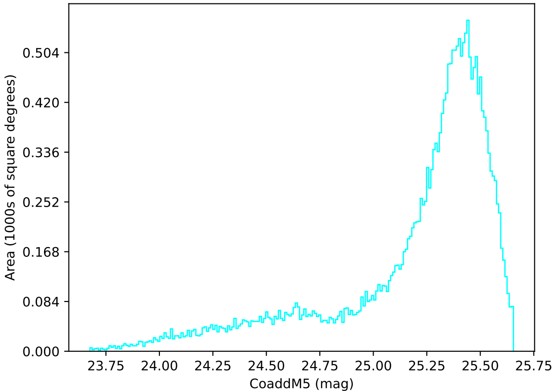
too_ignore_10_1v3.4_10yrs All sky u band: CoaddM5
