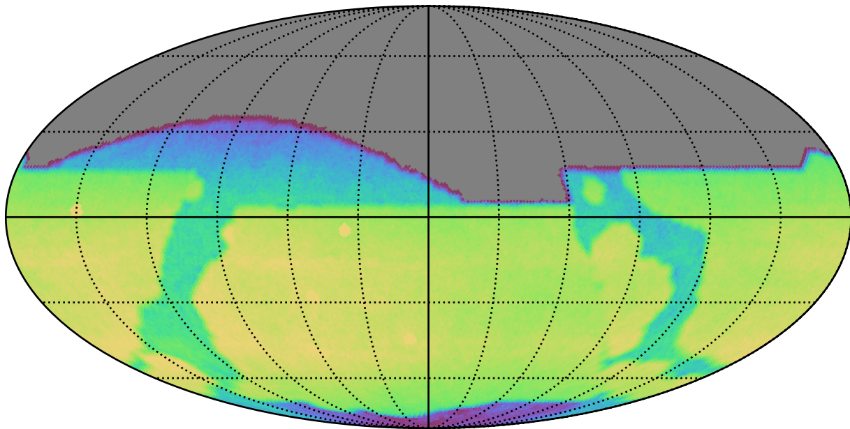
too_ignore_10_1v3.4_10yrs All sky r band: CoaddM5
