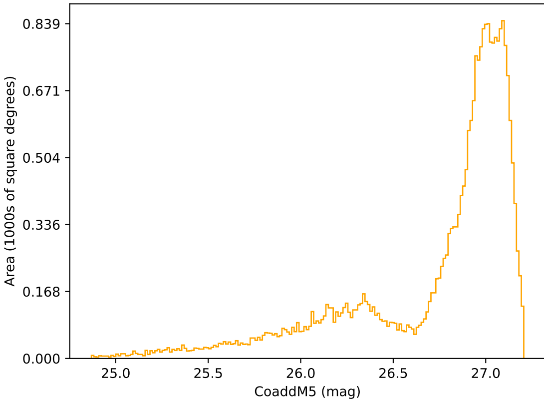
too_ignore_10_1v3.4_10yrs All sky r band: CoaddM5
