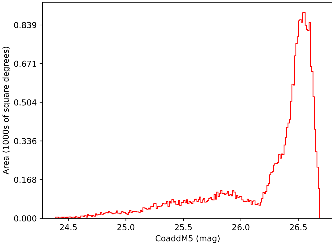
too_ignore_10_1v3.4_10yrs All sky i band: CoaddM5
