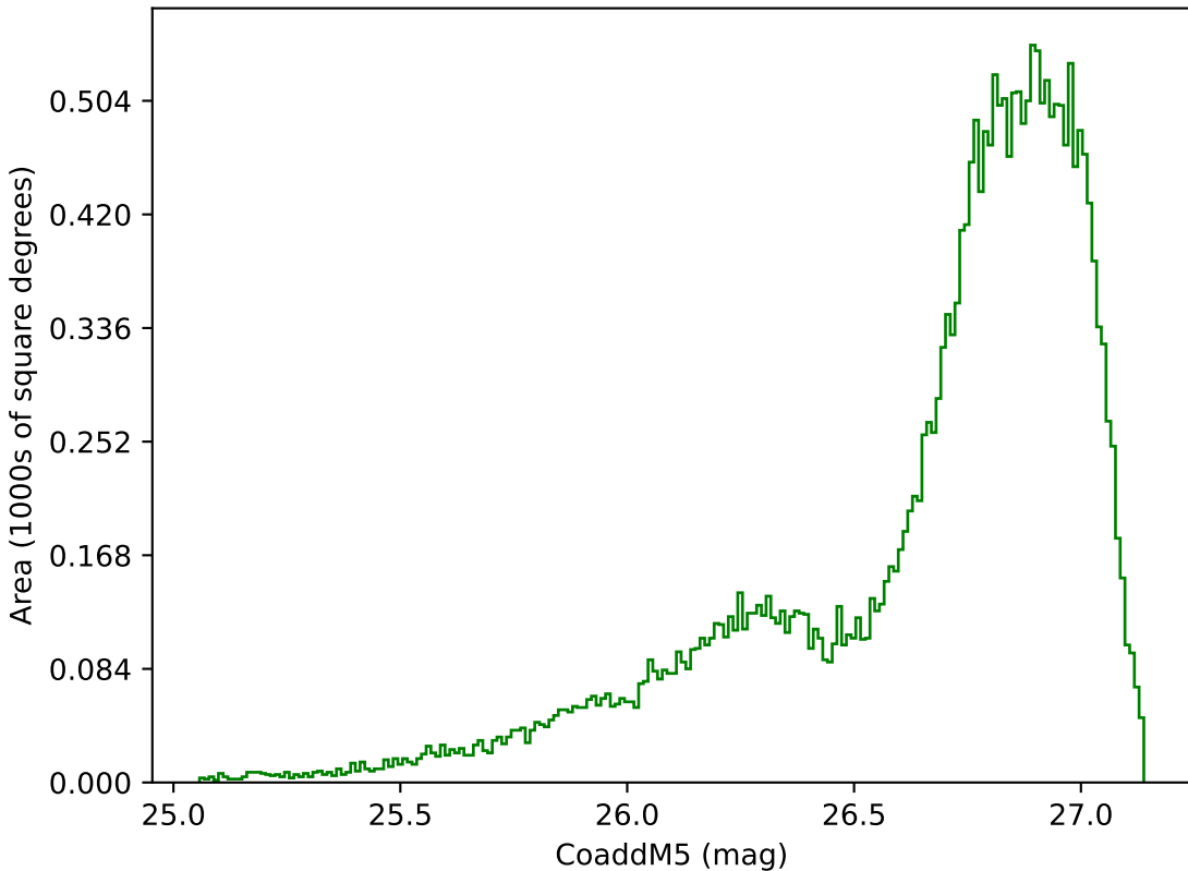
too_ignore_10_1v3.4_10yrs All sky g band: CoaddM5
