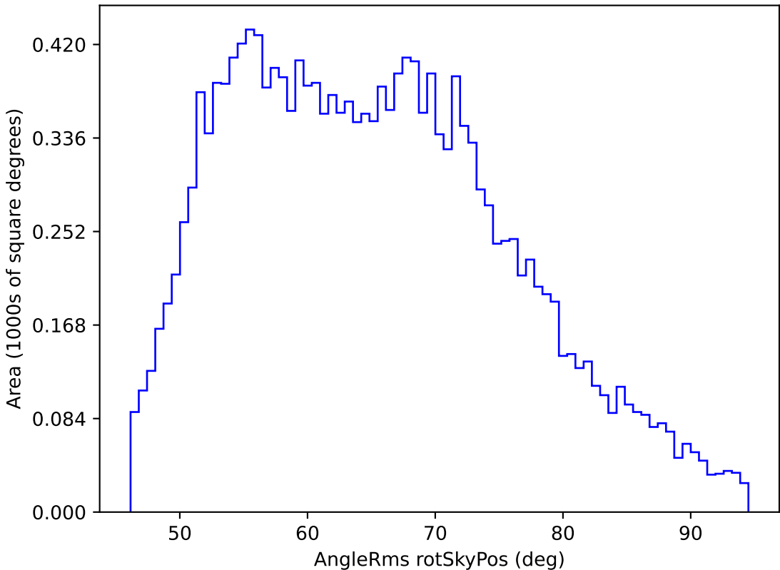
too_ignore_10_1v3.4_10yrs WFD u band: AngleRms rotSkyPos
