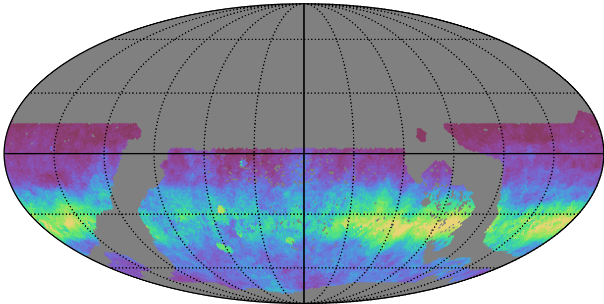
too_ignore_10_1v3.4_10yrs WFD r band: AngleRms rotSkyPos
