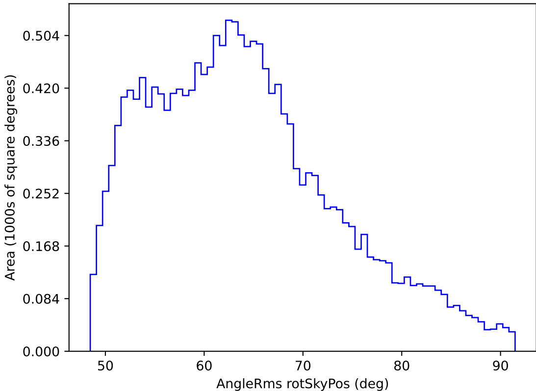
too_ignore_10_1v3.4_10yrs WFD i band: AngleRms rotSkyPos
