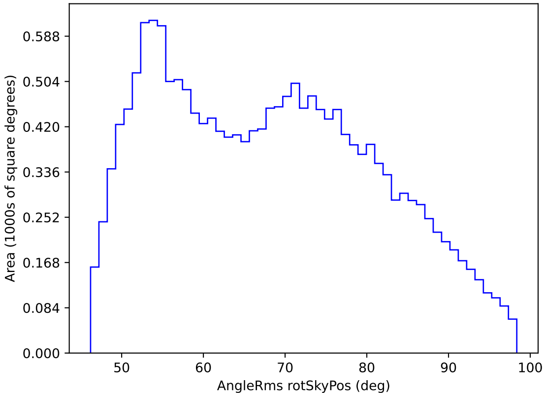
too_ignore_10_1v3.4_10yrs WFD g band: AngleRms rotSkyPos
