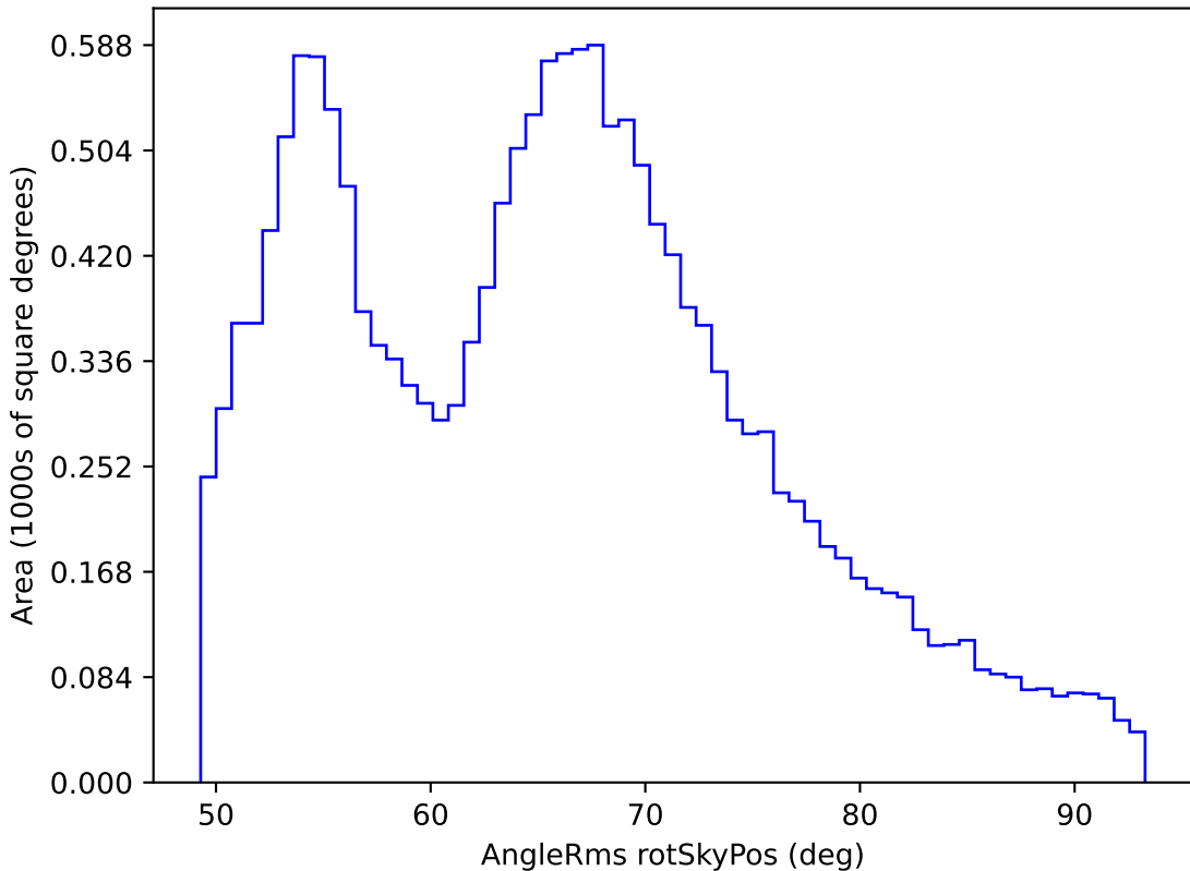
too_ignore_10_1v3.4_10yrs WFD all bands: AngleRms rotSkyPos
