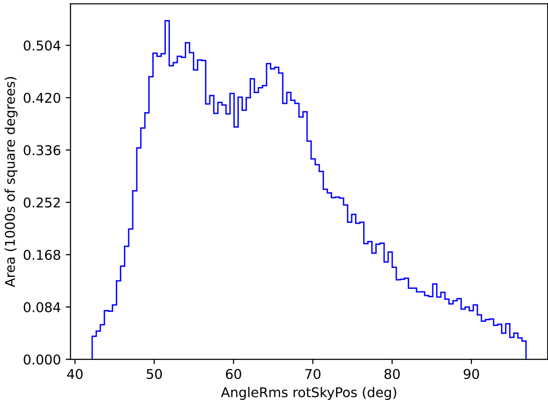
too_ignore_10_1v3.4_10yrs All sky r band: AngleRms rotSkyPos
